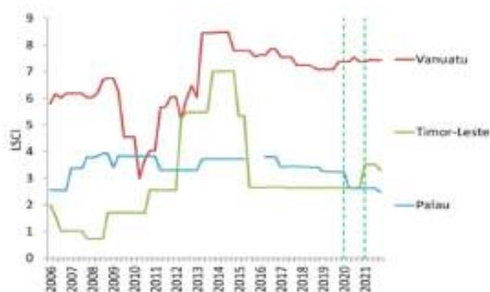
Figura 73: Evolusaun LSCI iha Timor-Leste no illa ki'ik sira balun (2006-2021)
